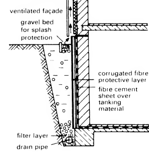
⑭ Protective layer of fibre cement boards
